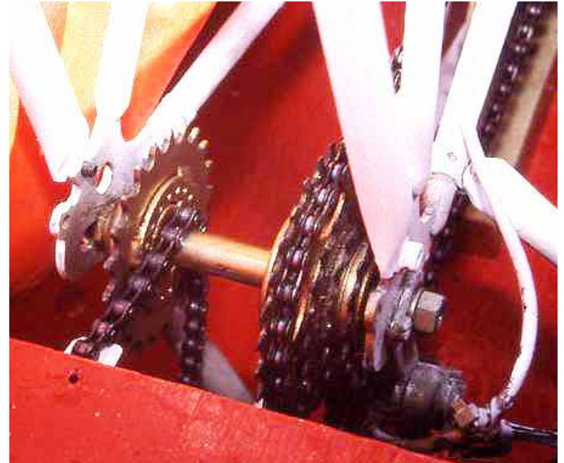
Misaligned sprockets caused this team endless derailments.
